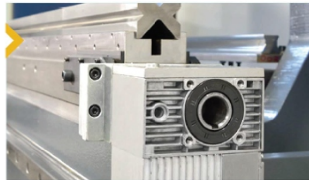
CNC controlled motorized crowning system - Option
